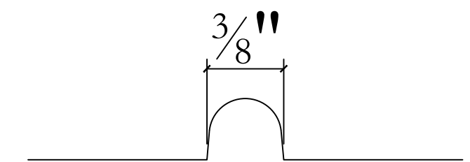
Typical Section
