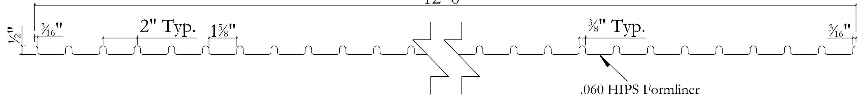
Typical Section 12'-0"
