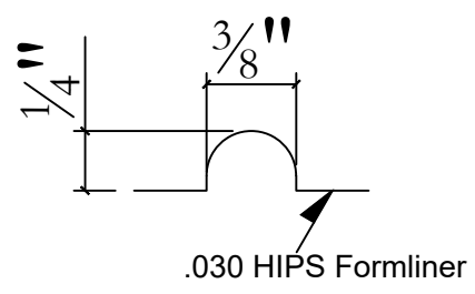
Typical Cove Joint Profile
