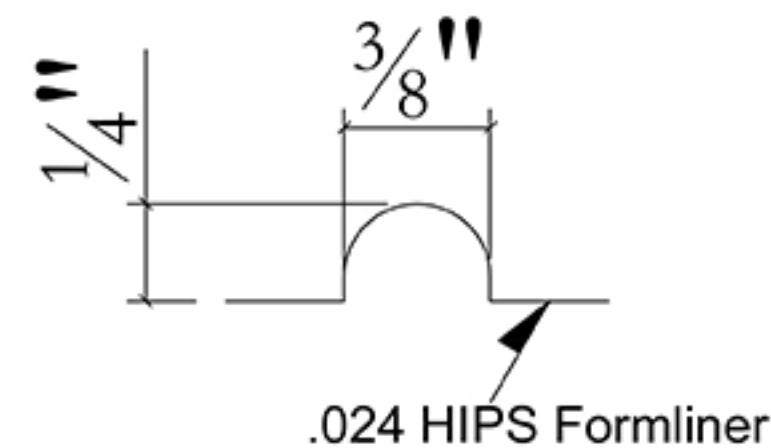
Typical Cove Joint Profile
