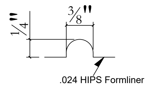
Typical Cove Joint Profile
