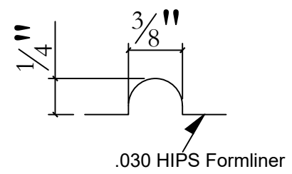
Typical Cove Joint Profile
