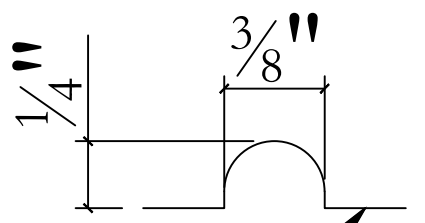
Typical Cove Joint Profile
