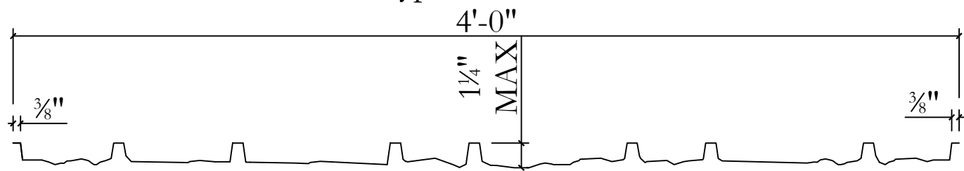
Typical section
