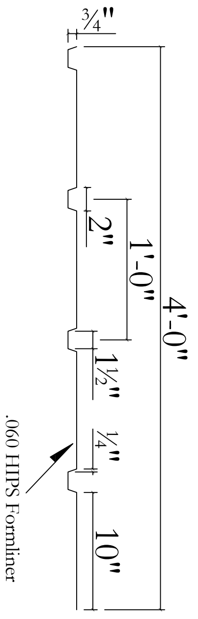
Typical Section
