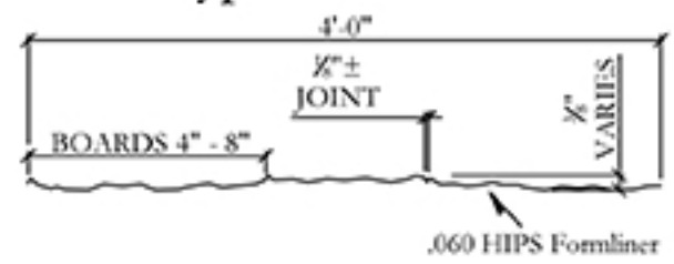
Typical Section
