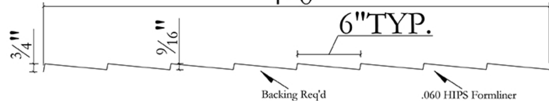
Wood Grain Texture Not Shown Typical Section 4'-0"
