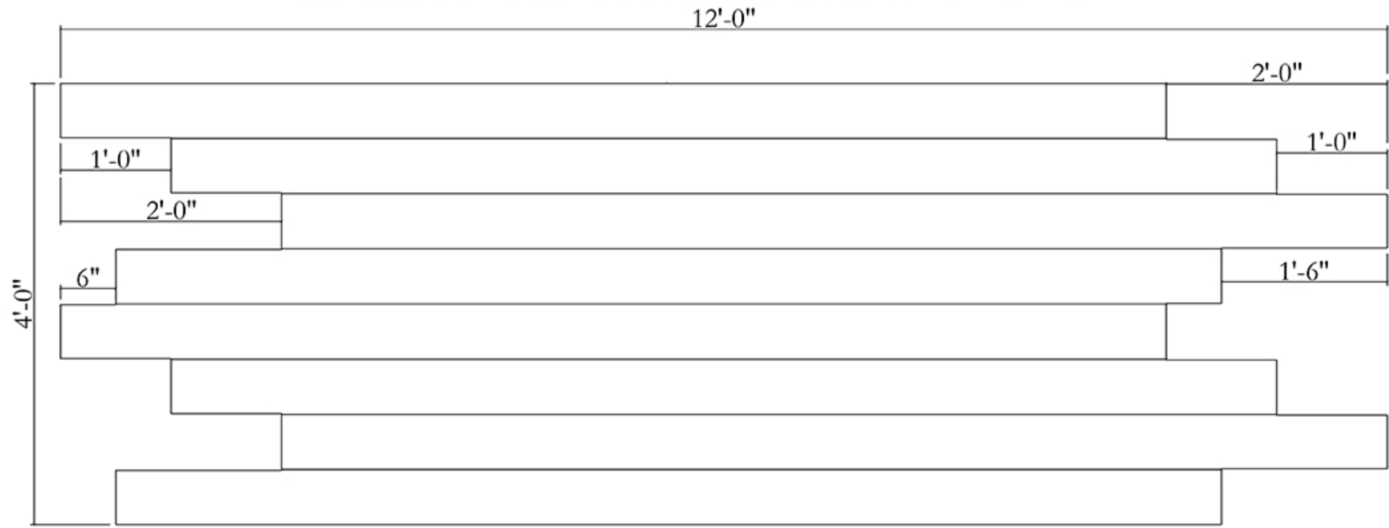
Wood Grain Texture Not Shown Typical Section 4'-0"
