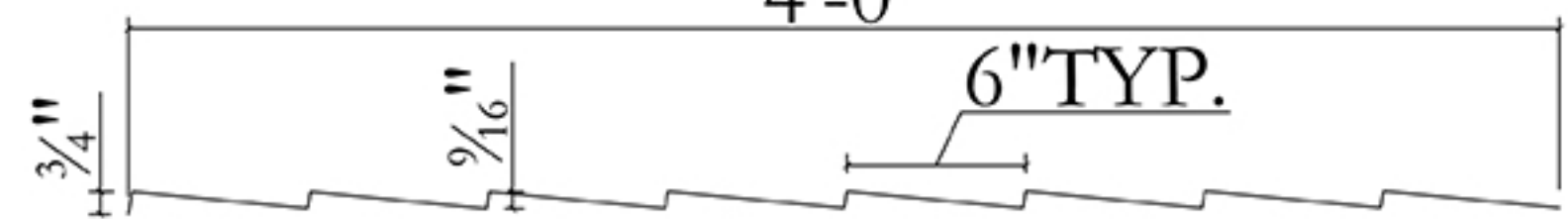
Typical Section 4'-0"
