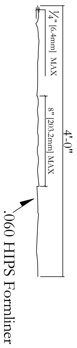
Typical Section
