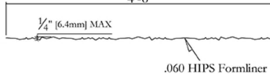
Typical Section 4'-0"
