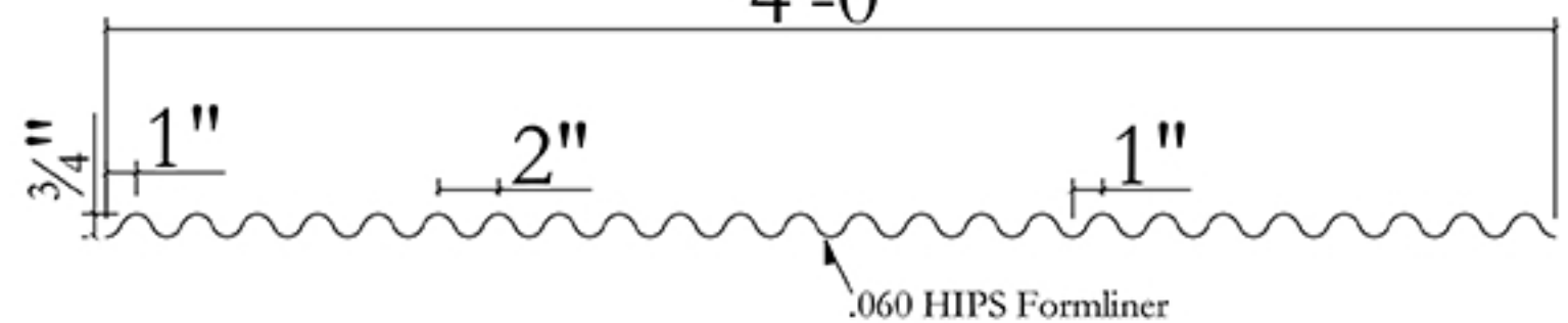
Typical Section 4'-0"
