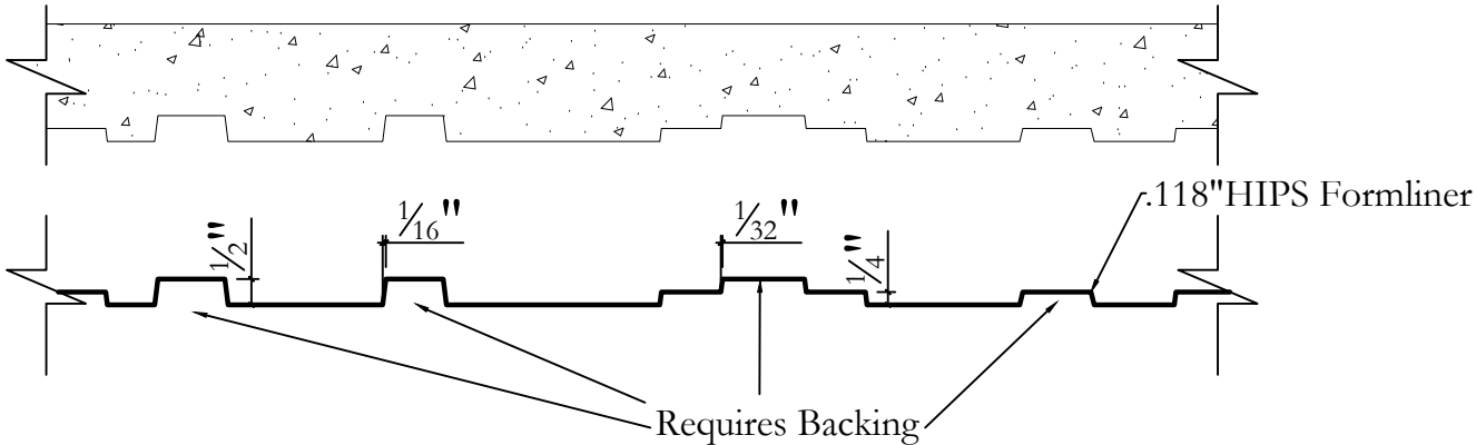
Typical Section
