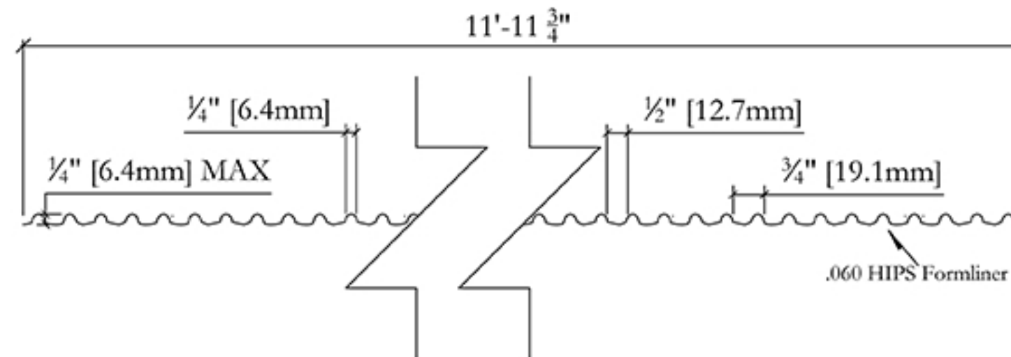
Typical Section
