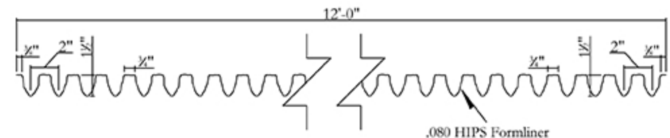
Typical Section
