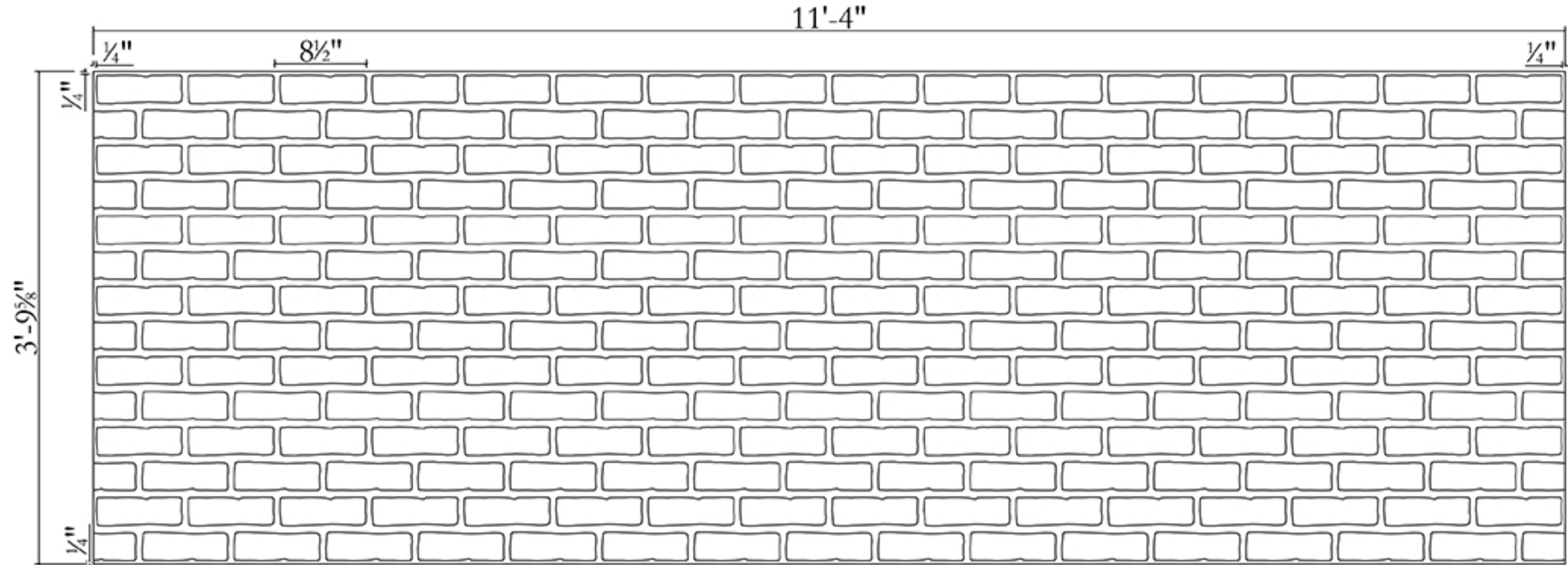
Typical Section
