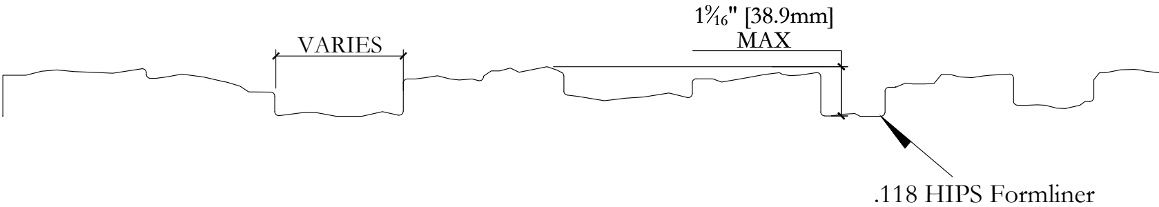
Typical Section
