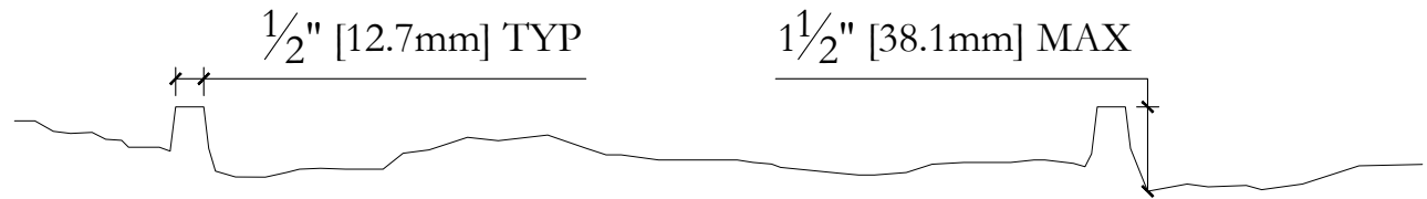
Typical section
