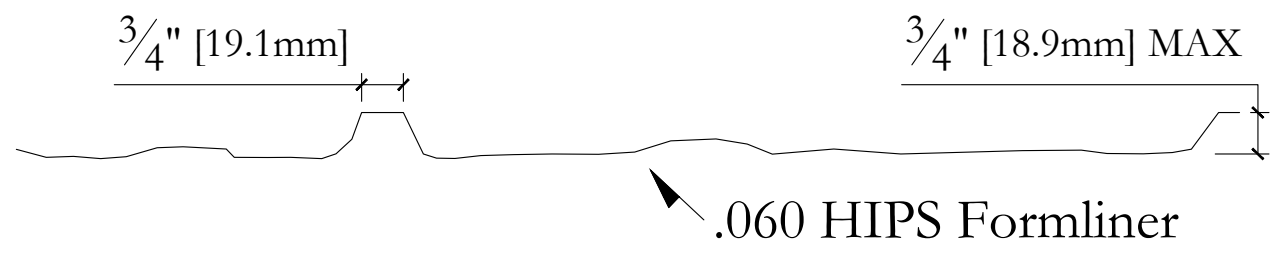
Typical Section
