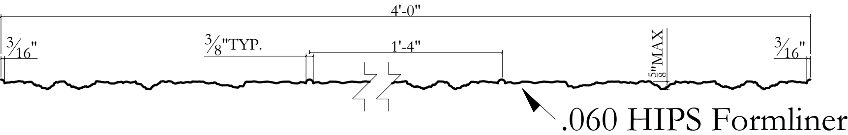
Typical Section
