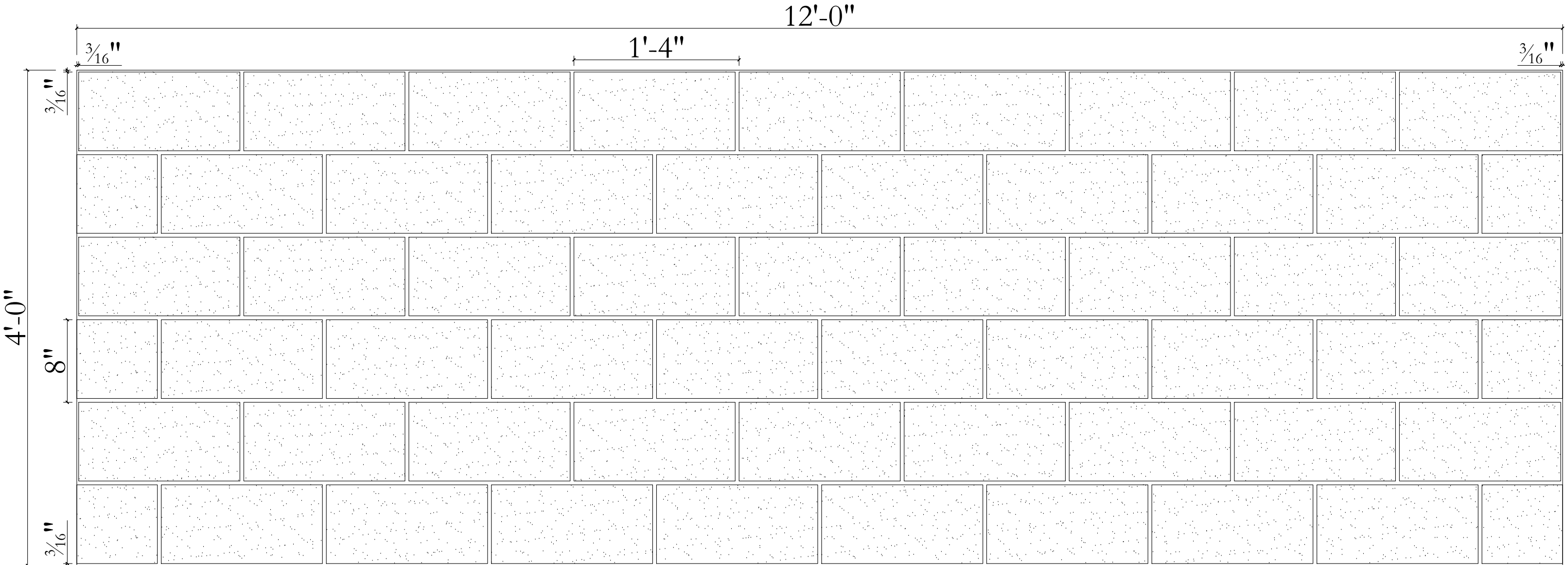
Typical Section
