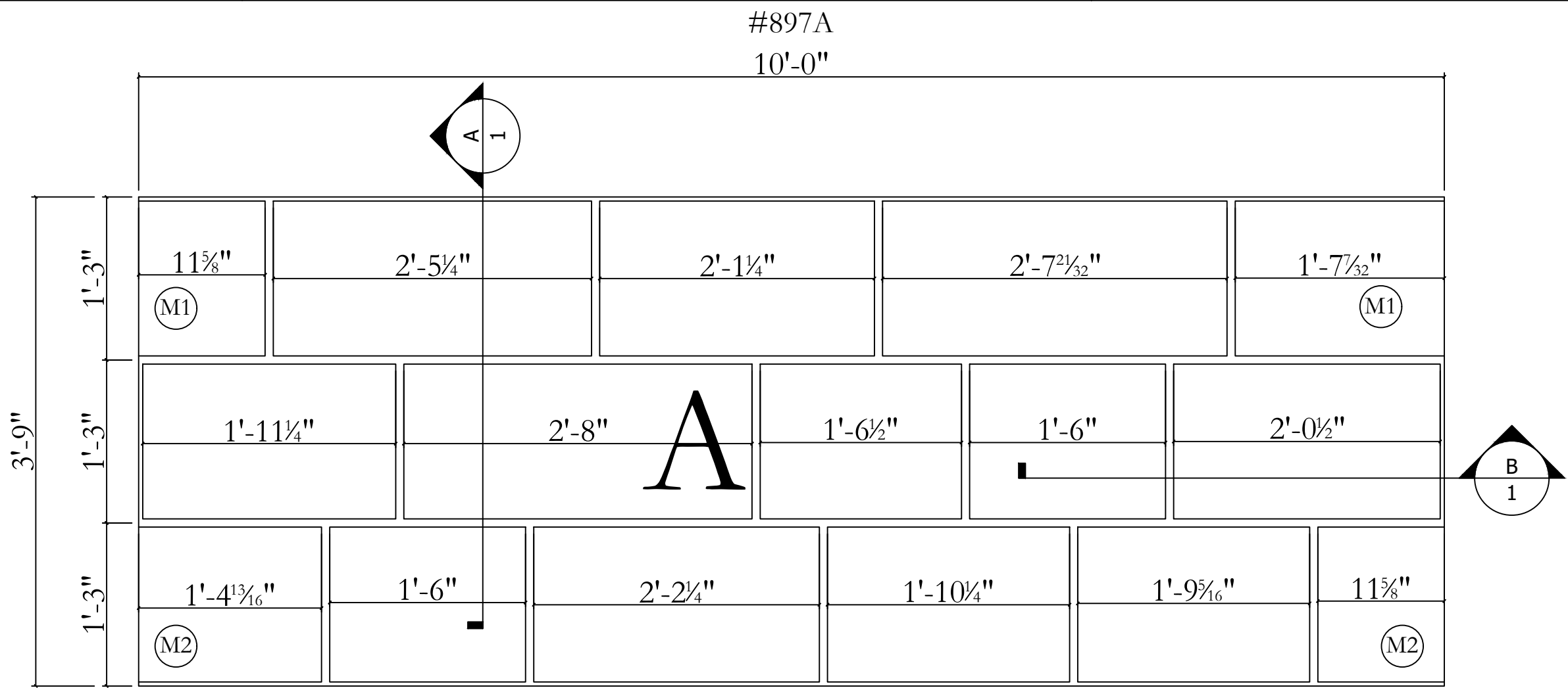
Stone Layout and Dimensions For Visual Reference Only Actual Stone Layout and Sizes May Vary
