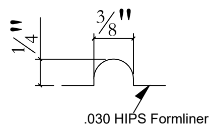
Typical Cove Joint Profile
