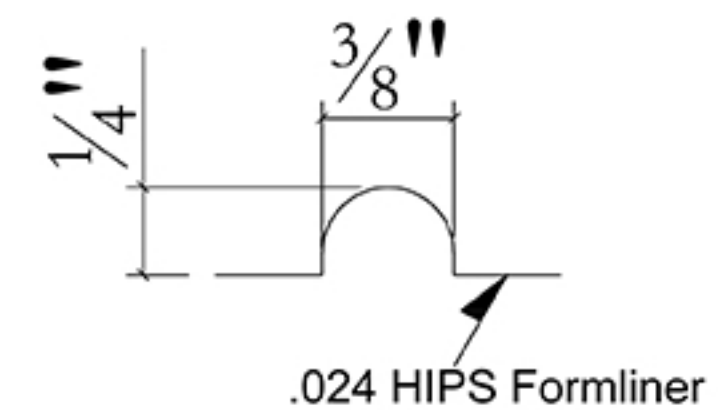
Typical Cove Joint Profile
