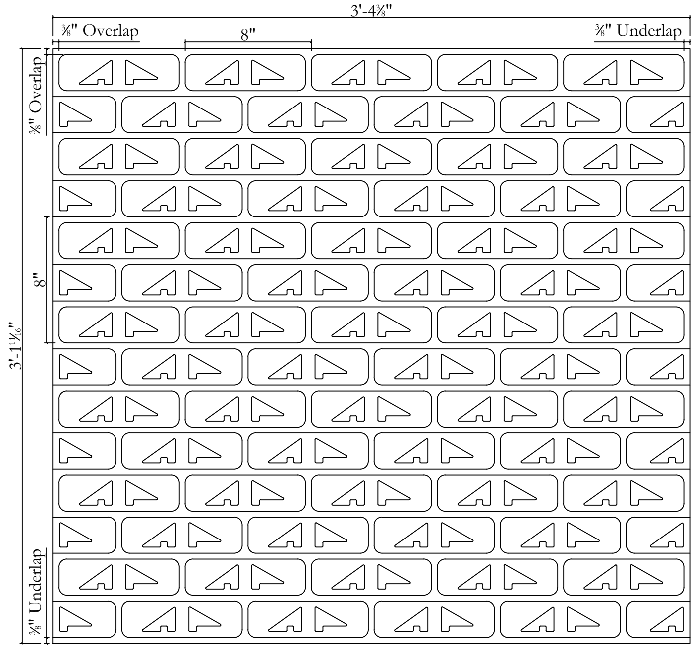
Typical Antique Classic Joint Profile
