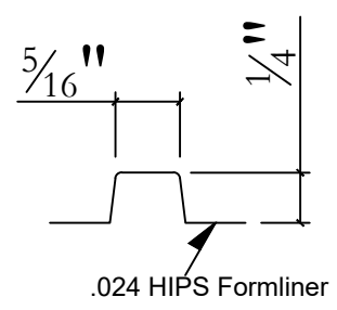
Typical Raked Joint Profile
