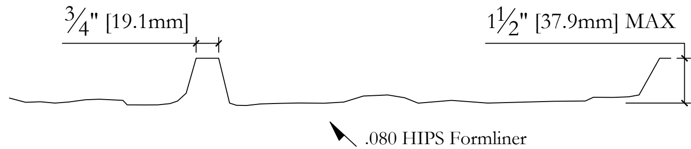
Typical Section
