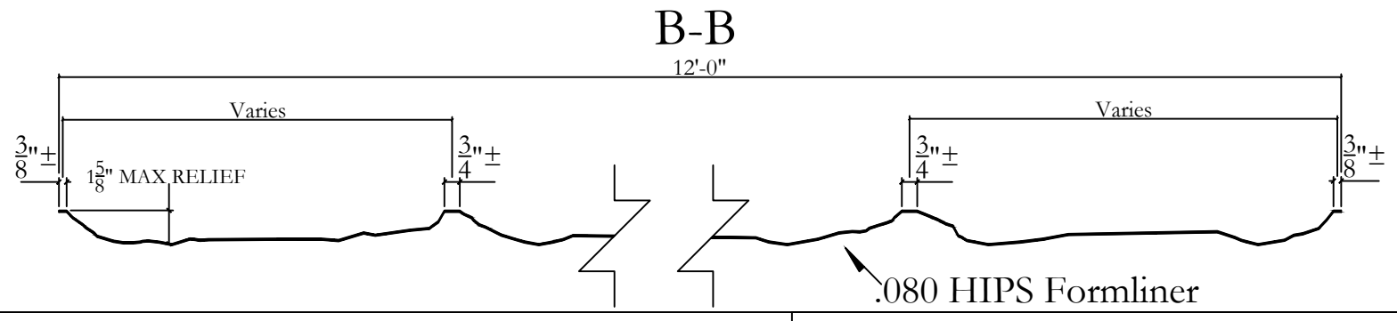
Stone Layout and Dimensions For Visual Reference Only Actual Stone Layout and Sizes May Vary
