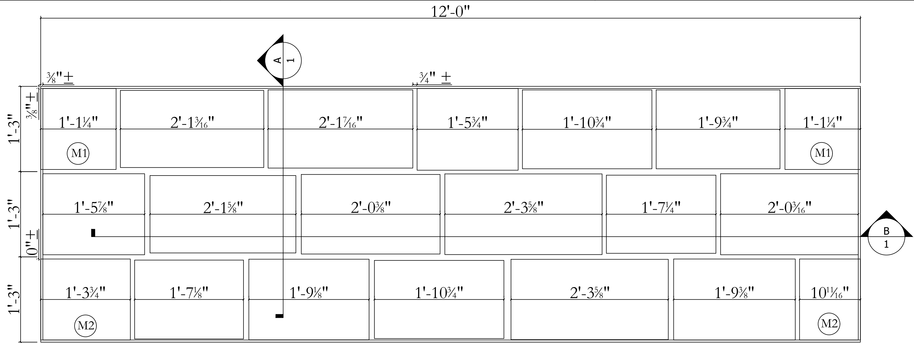
Stone Layout and Dimensions For Visual Reference Only Actual Stone Layout and Sizes May Vary
