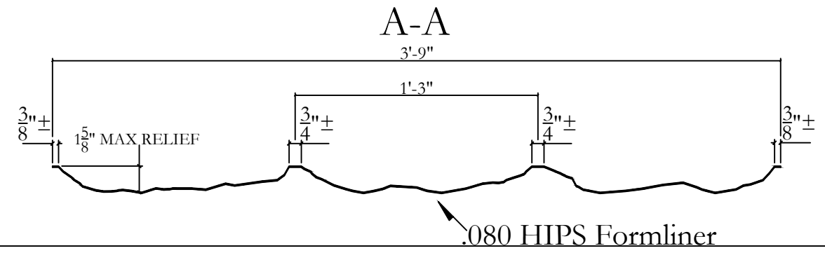
Stone Layout and Dimensions For Visual Reference Only Actual Stone Layout and Sizes May Vary
