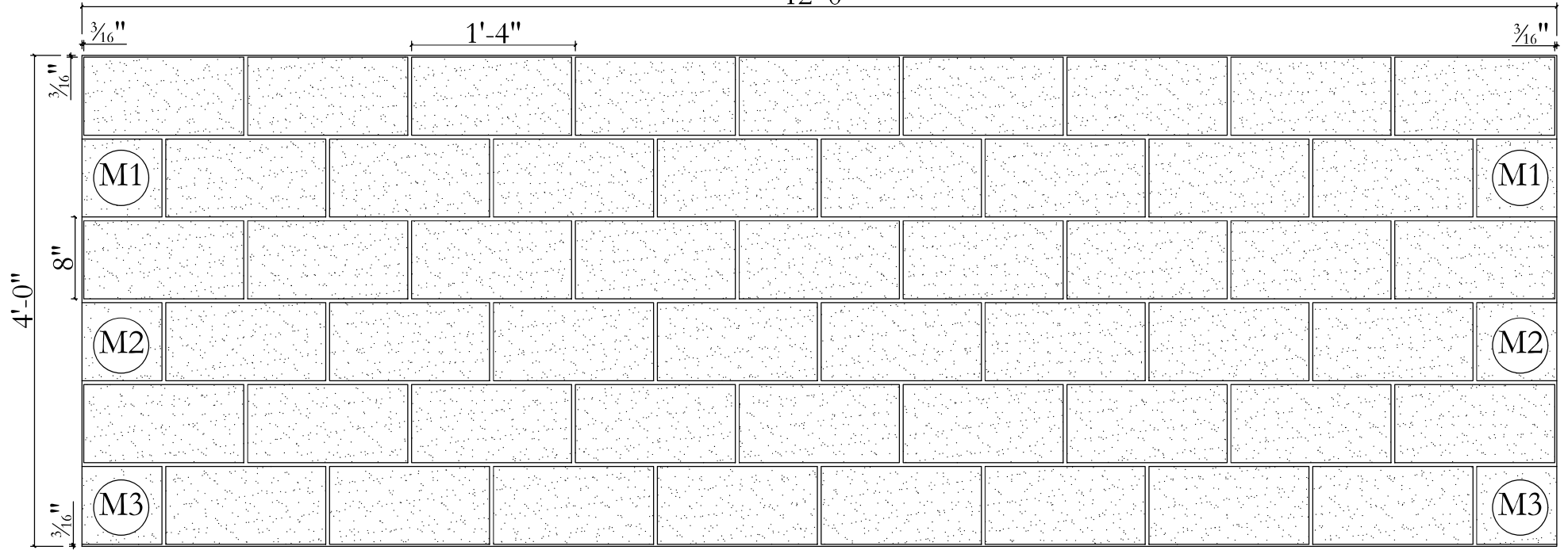
Typical Section
