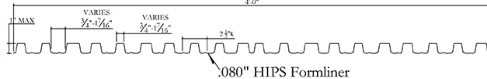
TYPICAL SECTION
