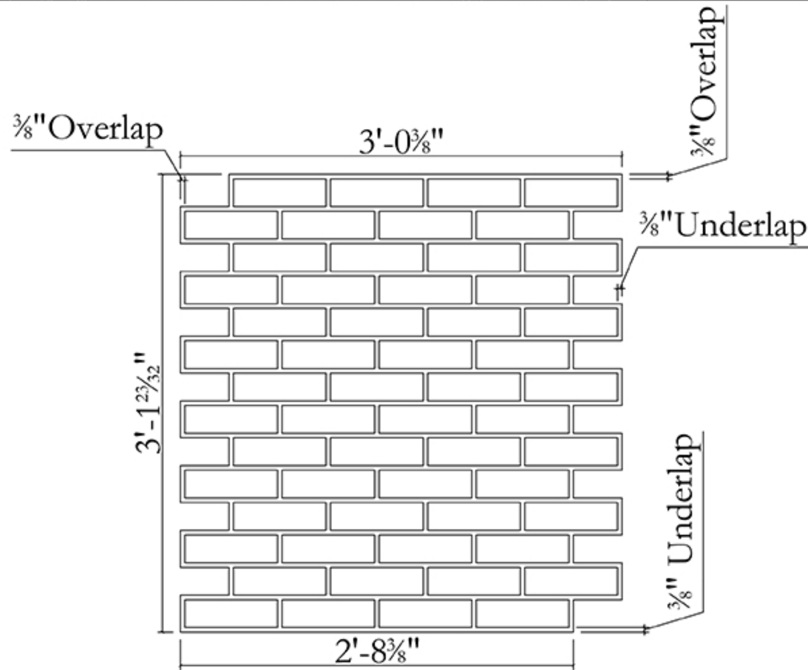
Typical Section
