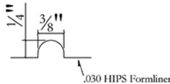
Typical Section
