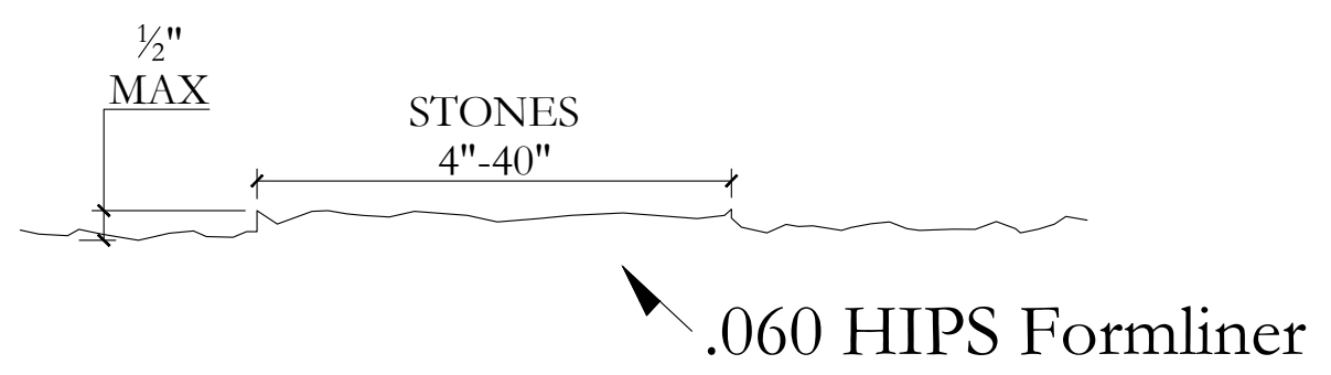
Typical Section
